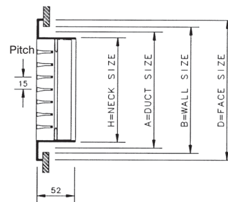
Sectional View
